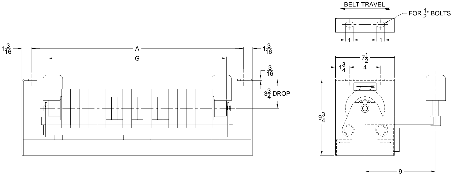
"ALL DIMENSIONS IN INCHES"
