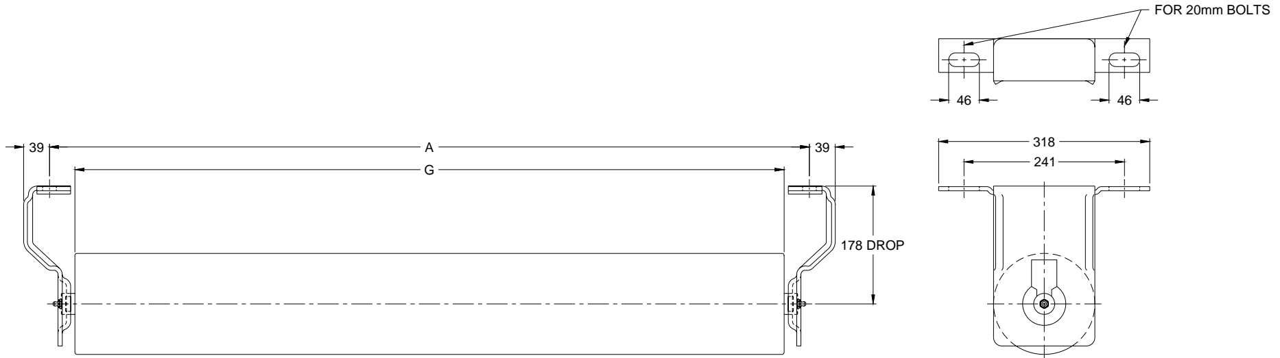
'Dimensions in Millimeters'
